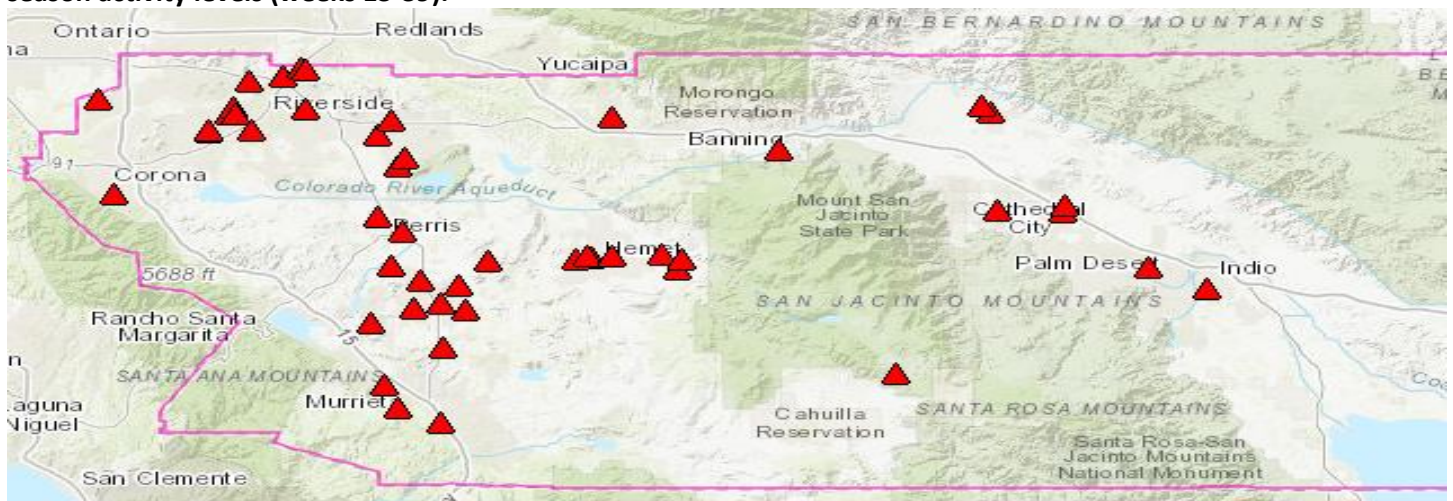
ILI-related EMS response in Riverside County, ePCR distribution map: Week 31
