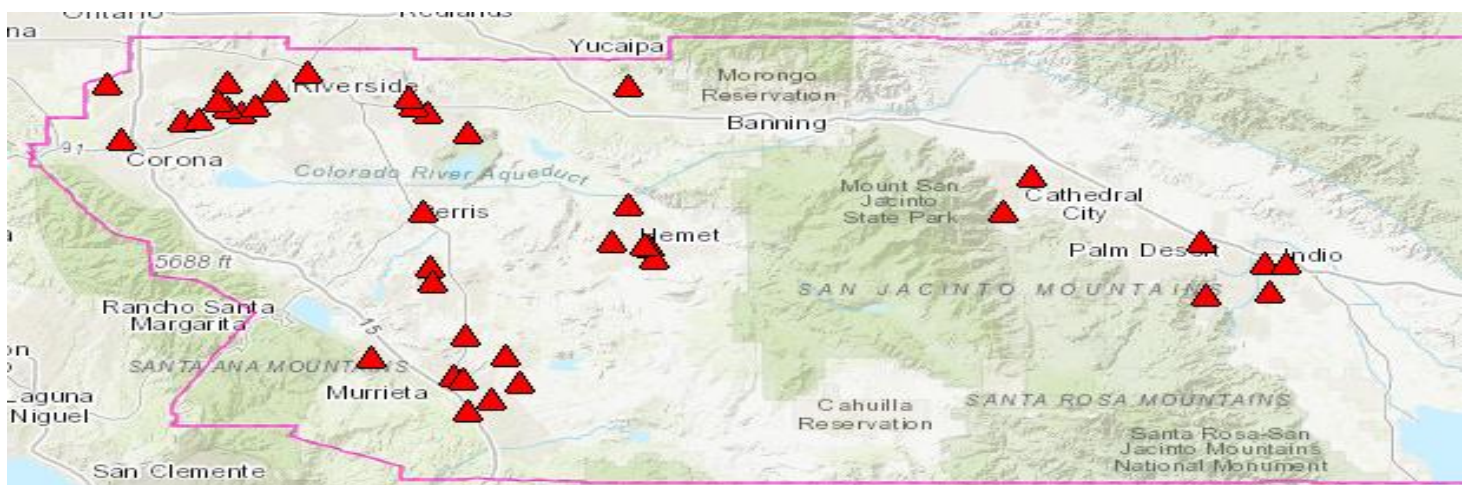
ILI-related EMS response in Riverside County, ePCR distribution map: Week 37
